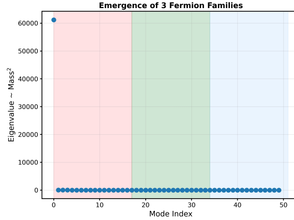
Figure 1: FIGURE 1: Emergence of 3 Fermion Families
