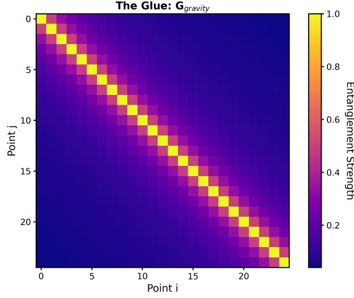
Figure 7: FIGURE 4: The Glue: G_{gravity}
