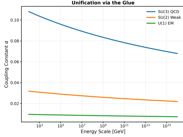
Figure 3: FIGURE 2: Unification via the Glue
