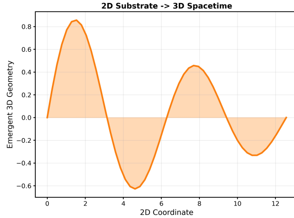
Figure 5: FIGURE 3: 2D Substrate -> 3D Spacetime
